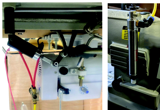
FOOTLIFT
