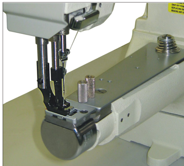
277RFS-3 Closeup showing synchronized binder arm, without binder attachment
