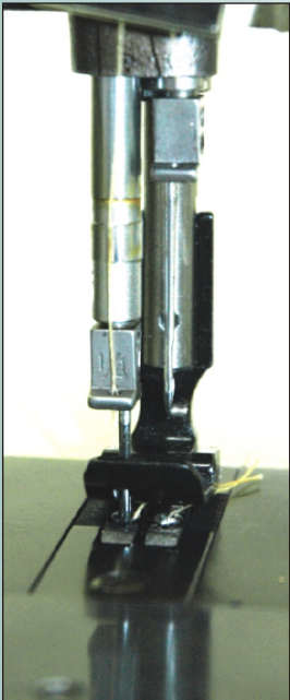
327RB-2 needle and foot closeup showing the split needle bar
