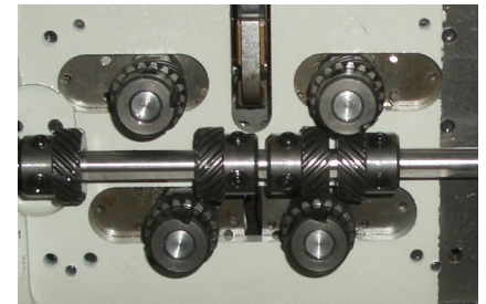
Adjustable gears allow use of any needle combination
