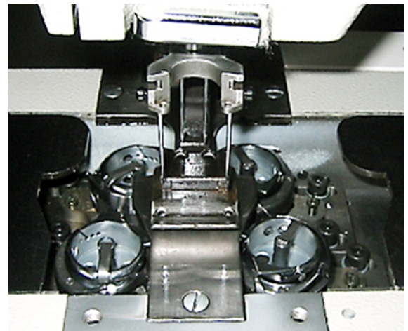
Four Horizontal Hooks and Bobbins
