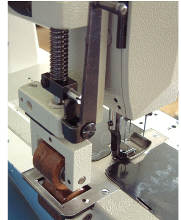
Puller Feeder
