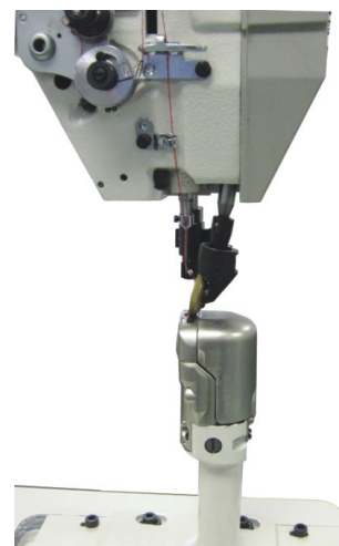
Closeup of 701LP Post and Needle
