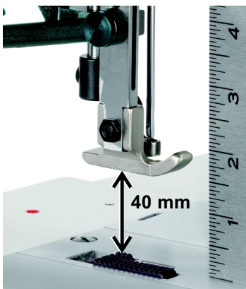
Detail of 733R-8 showing 40 mm extra high foot lift Single row feed with left half-foot
