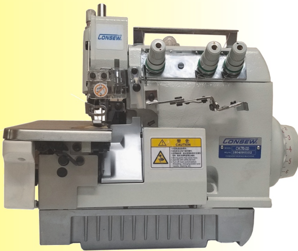
Stitch type 504
