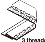
Stitch type 505
