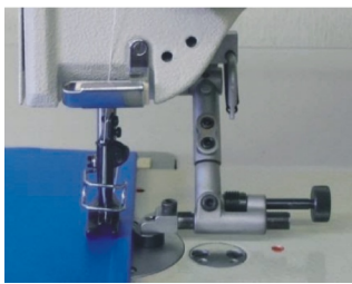
Back of P1510RB-14 showing the Footlift Air Lines and Air Cylinder.
