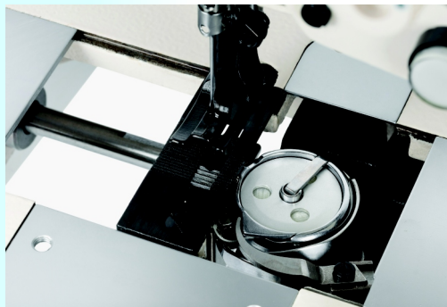
Top loading bobbin
