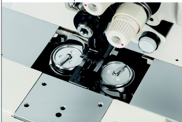
Two Top Load Bobbins
