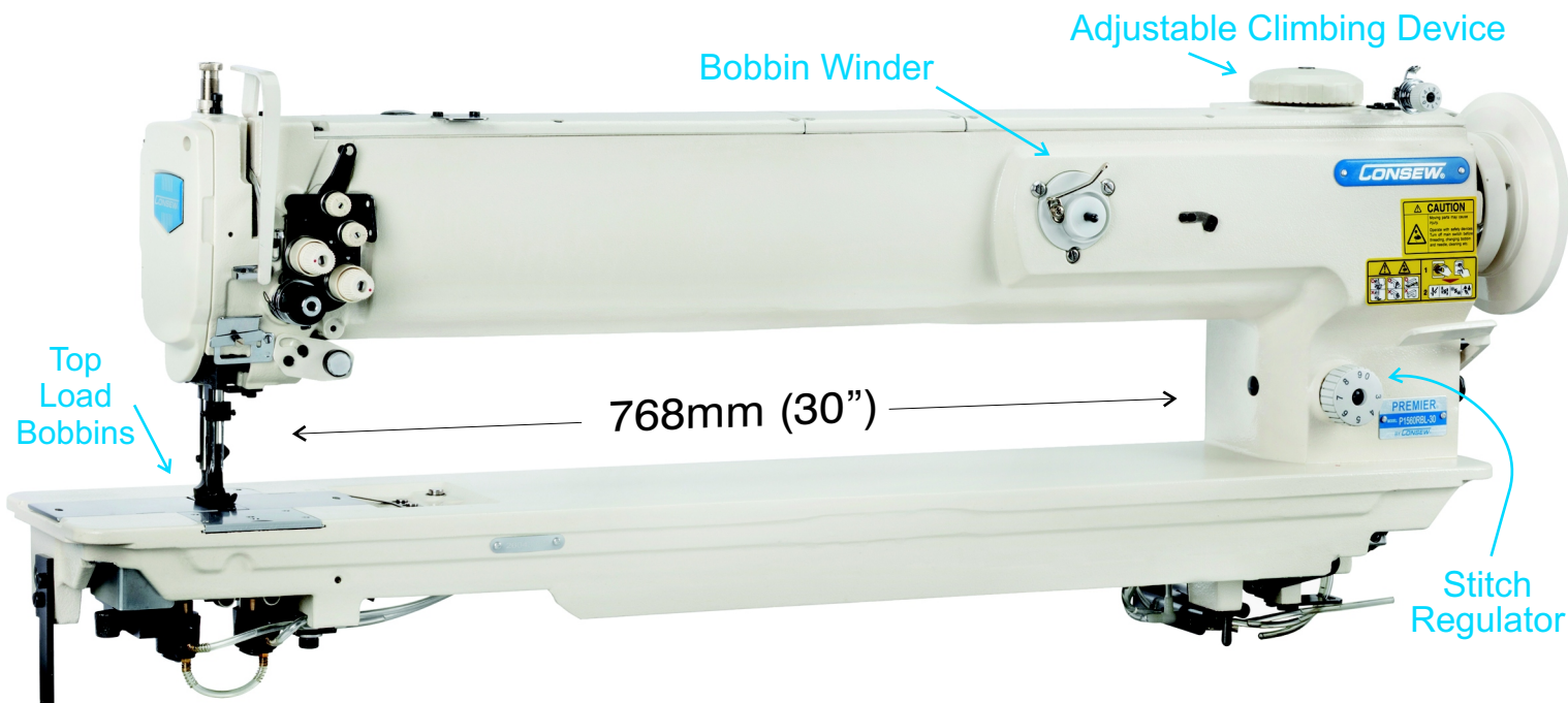
Two Top Load Bobbins
