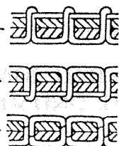
Fig. 24 - Perfect stitching. - Tight tension of needle thread. - Loose tension of needle thread.
