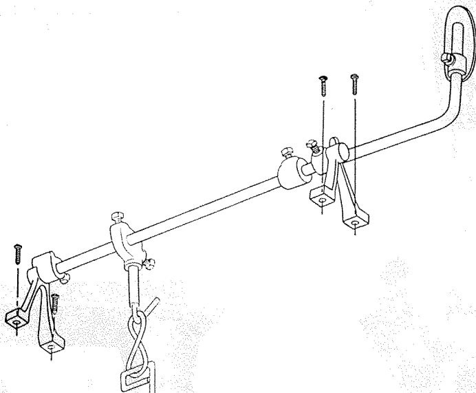
Fig. 6 To assemble the knee lifter (SKM-26 only)
